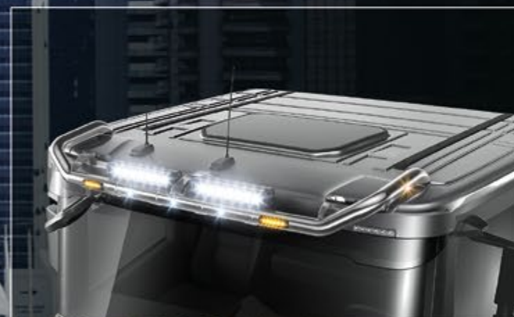
24706-3-P - LightFix - SKY-LIGHT Lightbar for mounting a maximum of 6 spotlights and 2 beacons stainless steel - polished - Ø 70mm - prewired
